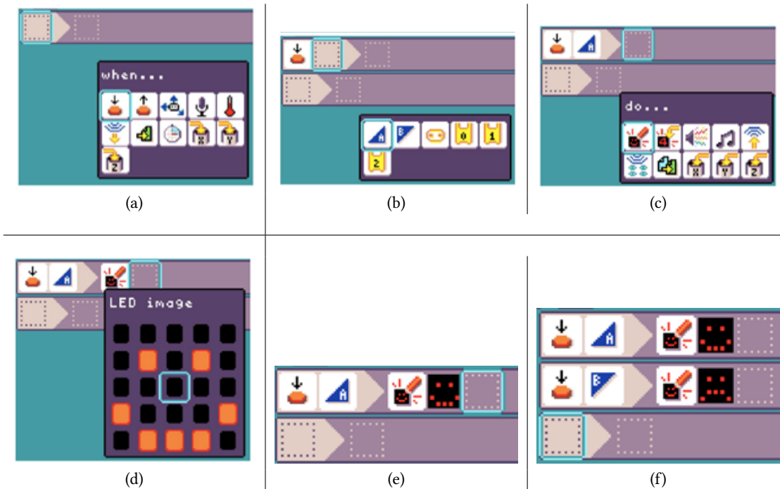
Fig. 5. (a-d) Editing actions to create a When-Do rule; (e) resulting rule; (f) addition of second rule.
