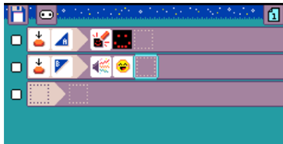
Fig. 7. A sample MicroCode program the teacher demonstrated to the students.
