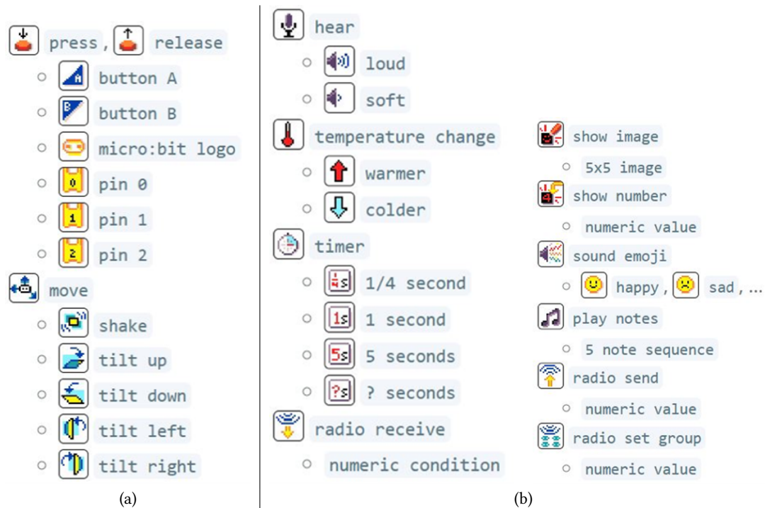
Fig. 4. MicroCode programming tiles for (a) events and (b) actions. Images were designed to represent the physical hardware.
